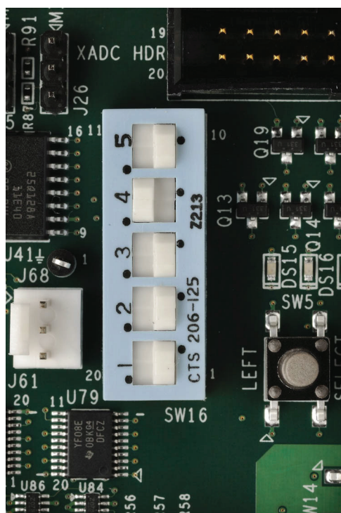
Figure 2-1: Settings for the Mode Switch to Boot from Quad SPI Mode
