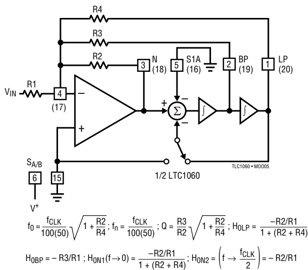
Figure 8. Mode 2: 2nd Order Filter Providing Notch, Bandpass, Lowpass
