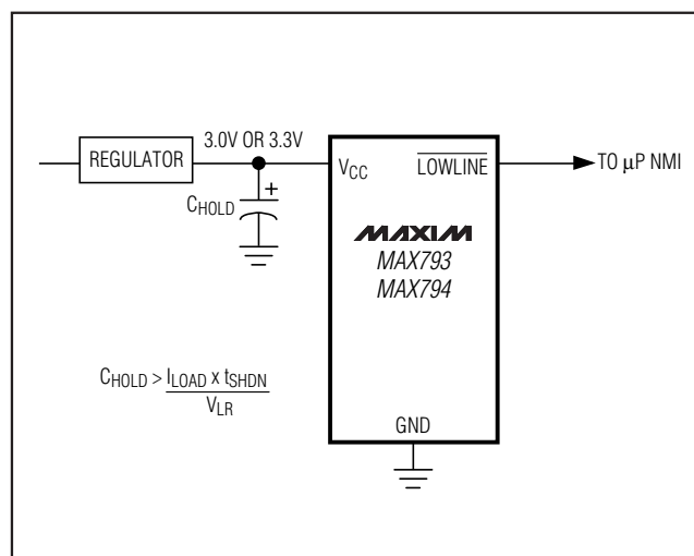
Figure 11. Using LOWLINE to Provide Power-Fail Warning to the \mu P
