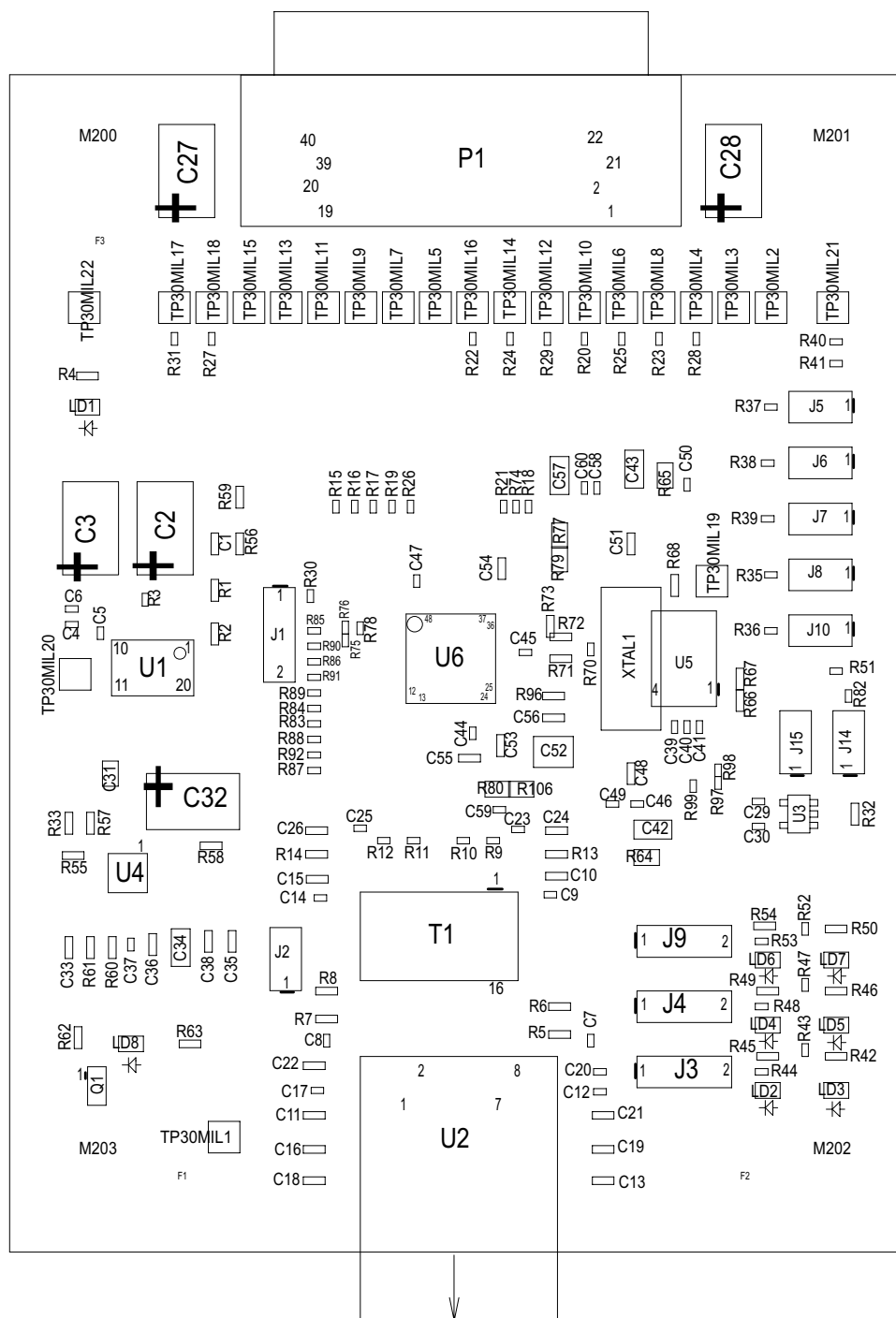
Figure 2. EVM Layout
