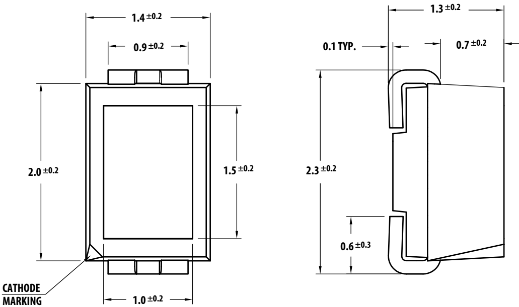
Figure 1: Package Drawing
