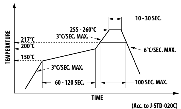
Figure 11: Recommended Pb-Free Soldering Profile
