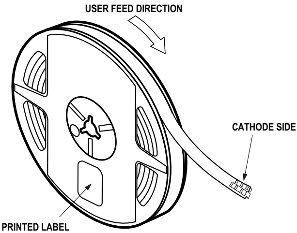
Figure 14: Reeling Orientation
