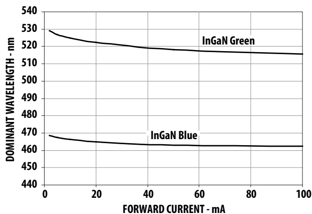
Figure 7: Dominant Wavelength Shift vs. Forward Current
