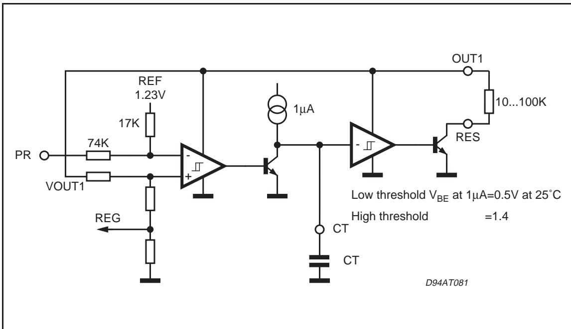
Figure 3: Reset Generator
