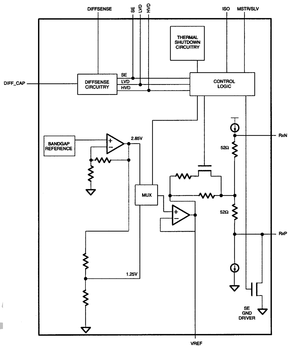
Figure 1. DS2117M Block Diagram
