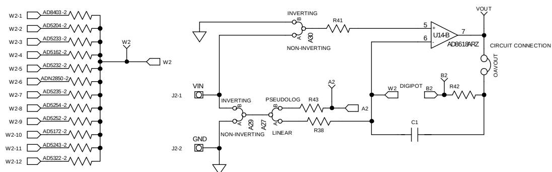
Figure 13. Schematic of Multiboard RDAC1 Circuits
