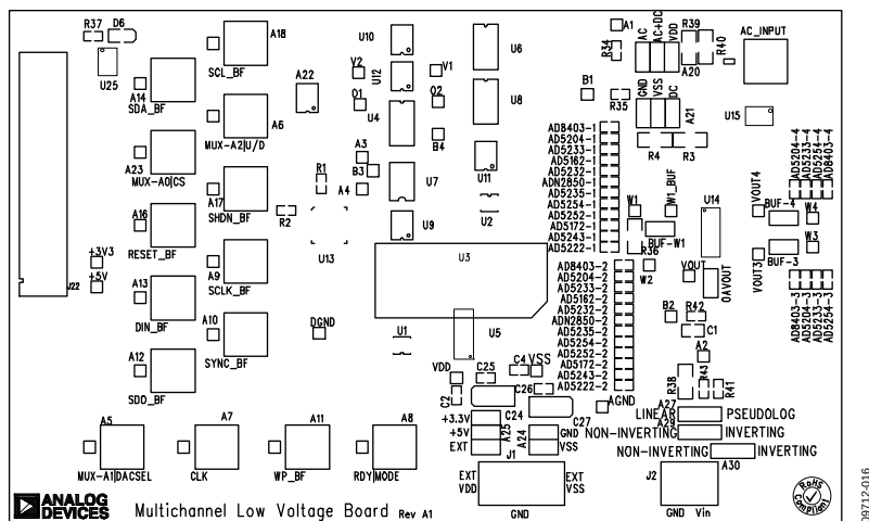
Figure 16. Component Side View
