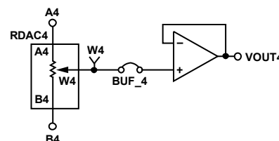
Figure 8. RDAC4 Output Buffer
