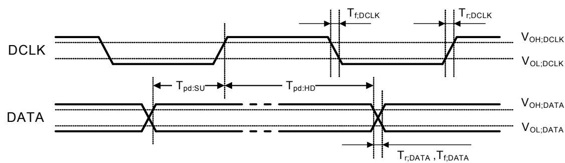
Figure 11 DCLK and DATA out
