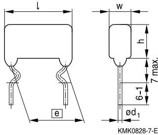
Straight leads
