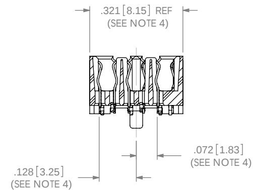
SECTION "F"-"F"
