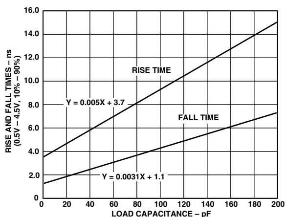
Figure 28. Typical Output Rise Time (10%–90% V_{DD} ) vs. Load Capacitance ( V_{DD} = 5\text{ V} )
