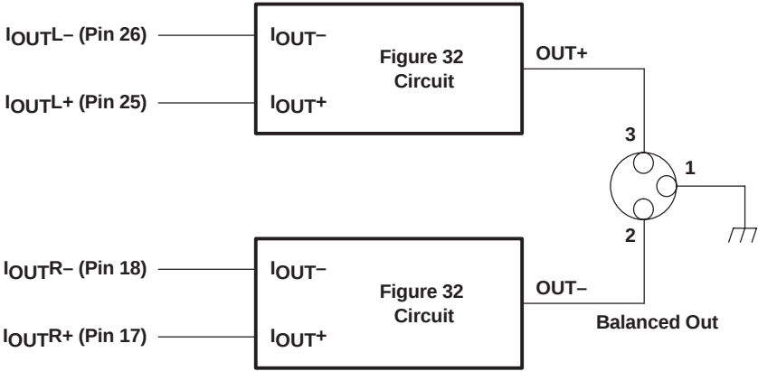
Figure 34. Measurement Circuit for Monoaural Mode
