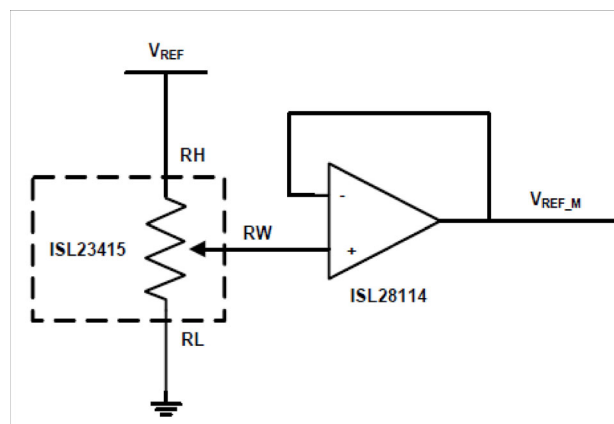
FIGURE 2. V_{\text{REF}} ADJUSTMENT
