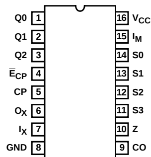
HD-4702 (CERDIP, PDIP) TOP VIEW
