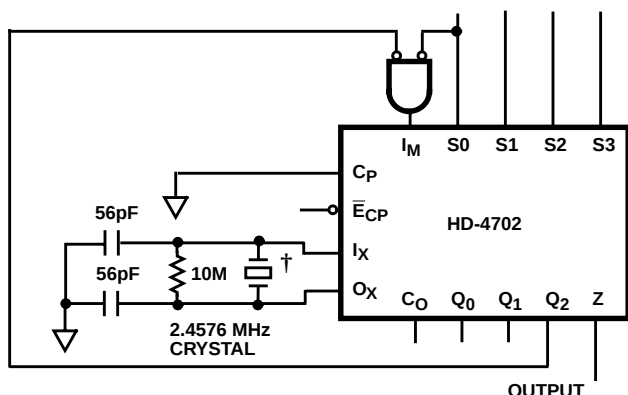
FIGURE 3. 19200 BAUD OPERATION
