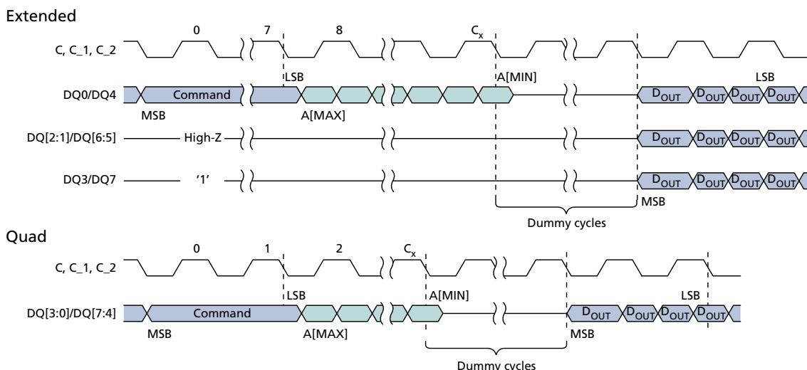
Figure 27: DTR QUAD OUTPUT FAST READ – 6Dh
