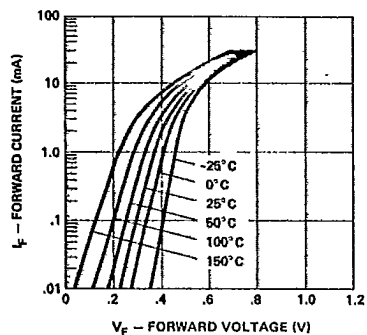
Figure 10. I-V Curve Showing Typical Temperature Variation for the 5082-2811 Schottky Diode.
