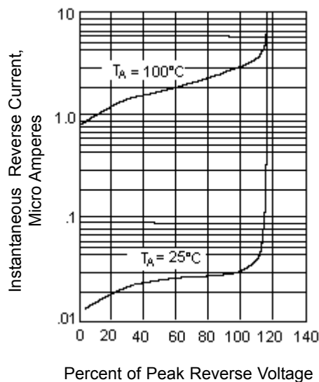
Figure 4 - Typical Reverse Leakage Characteristics per Leg
