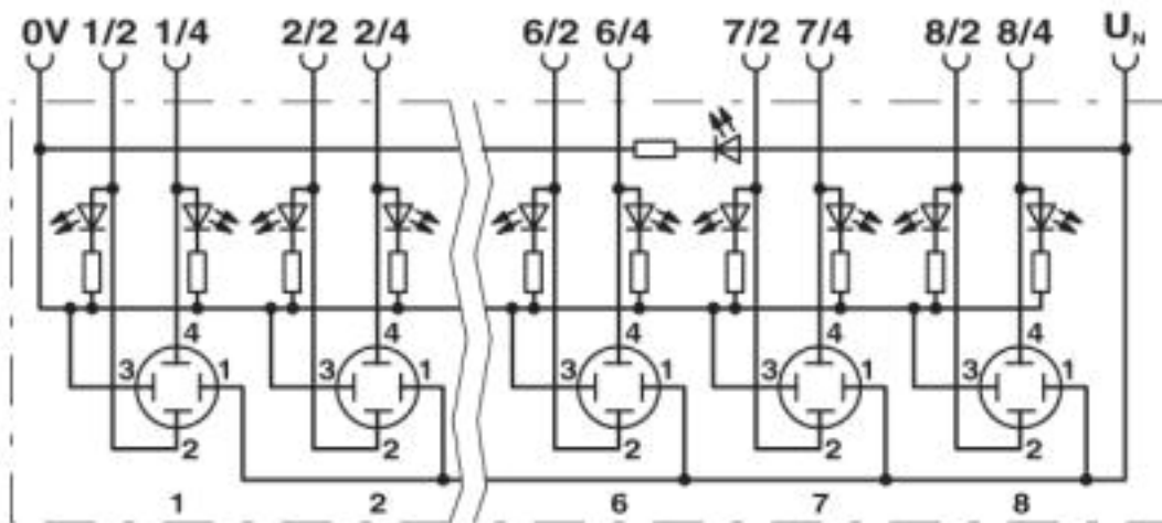
Circuit diagram
