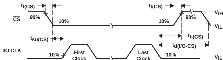
Figure 10. \overline{\text{CS}} and I/O CLK Voltage Waveforms
