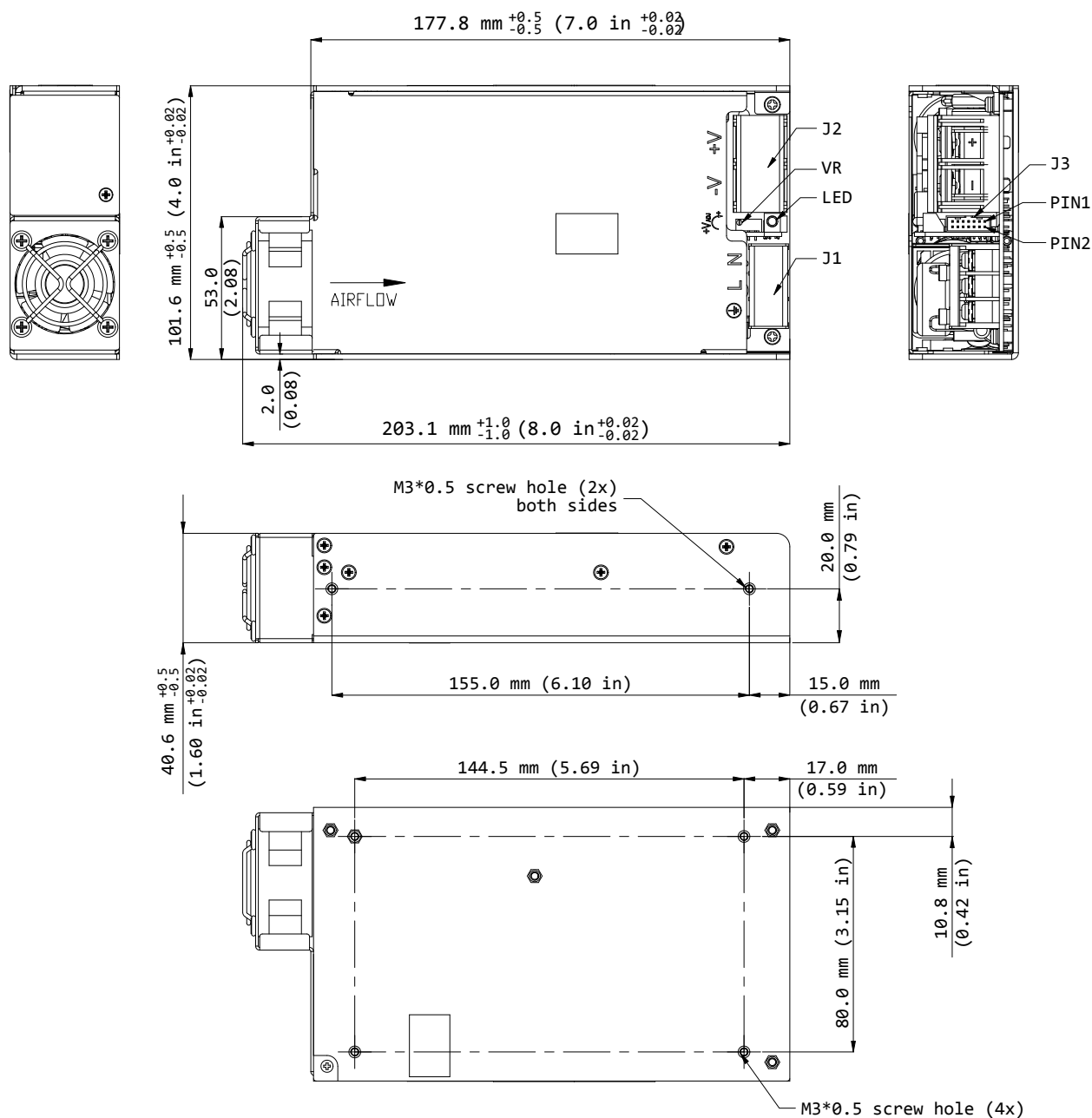
Fig. 6: Dimensional drawing IMA-x600-xx
