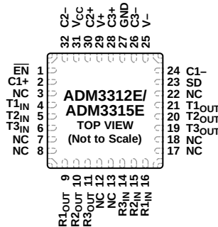
Figure 6. LFCSP_WQ Pin Configuration
