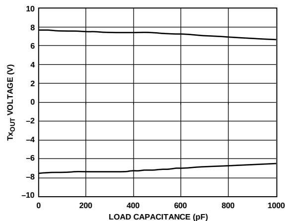
Figure 20. Transmitter Output Voltage High/Low vs. Load Capacitance ( V_{CC} = 3.3 \text{ V} , CLK = 1 Mb/s, R_L = 5 \text{ k}\Omega , ADM3307E)
