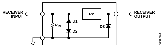
Figure 32. ADM3307E Receiver Input Protection Scheme
