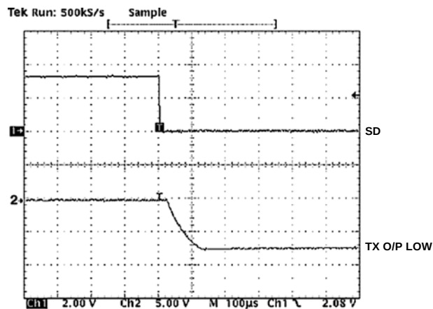
Figure 19. Transmitter Output (Low) Exiting Shutdown
