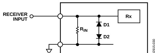
Figure 30. Receiver Input Protection Scheme
