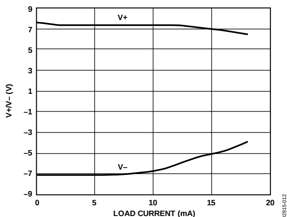
Figure 12. Charge Pump V+/- vs. Load Current ( V_{CC} = 3.3 V)
