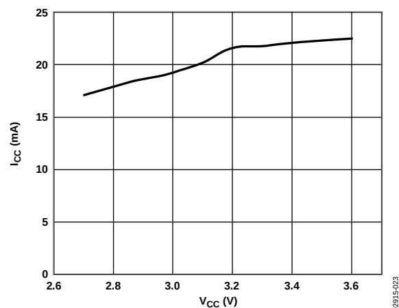
Figure 23. I_{CC} vs. V_{CC} ( R_L = 3\text{ k}\Omega )
