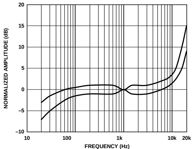
Figure 3. Frequency Response Mask
