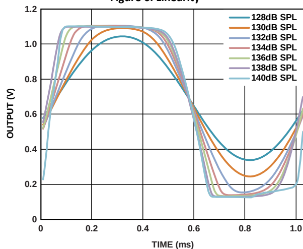
Figure 8. Clipping Characteristics
