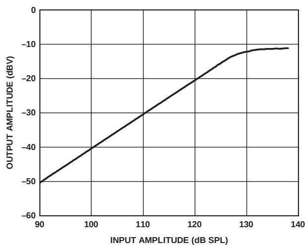
Figure 6. Linearity
