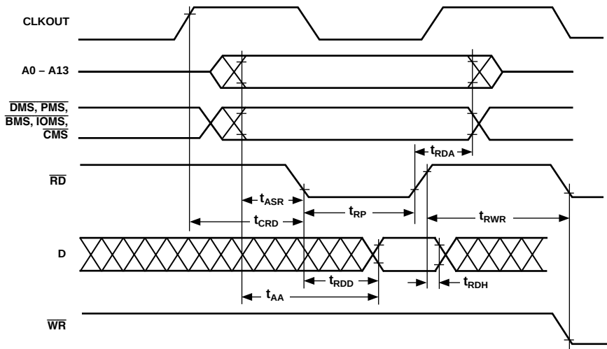
Figure 12. Memory Read
