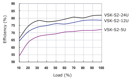
efficiency vs. output power (Vin=230 Vac)
