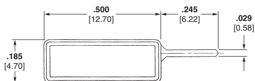
Polarizing Key 1-1437023-2
