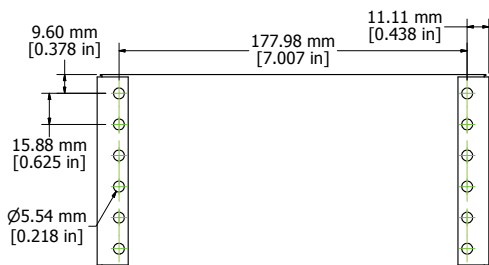
END PLATES
