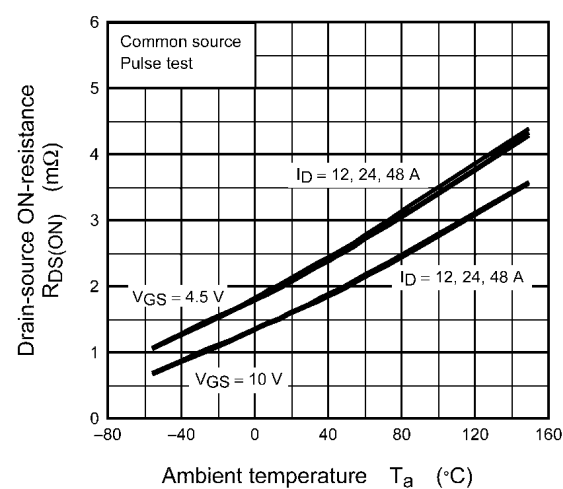
Fig. 8.6 R_{DS(ON)} - T_a
