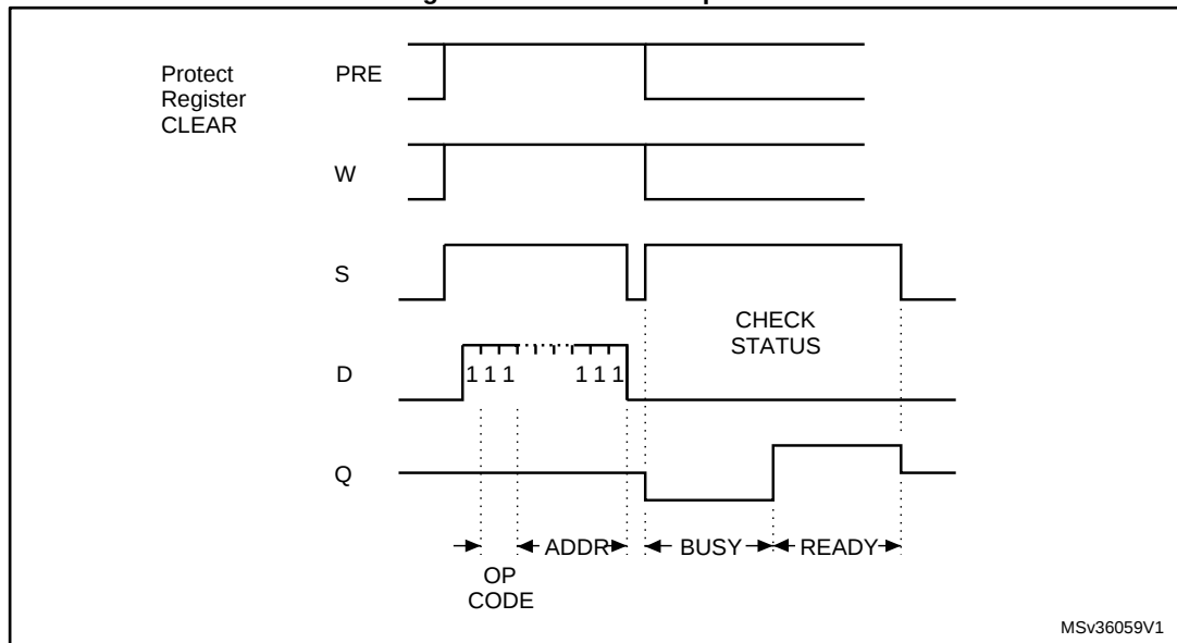
Figure 12: PRCLEAR sequence
