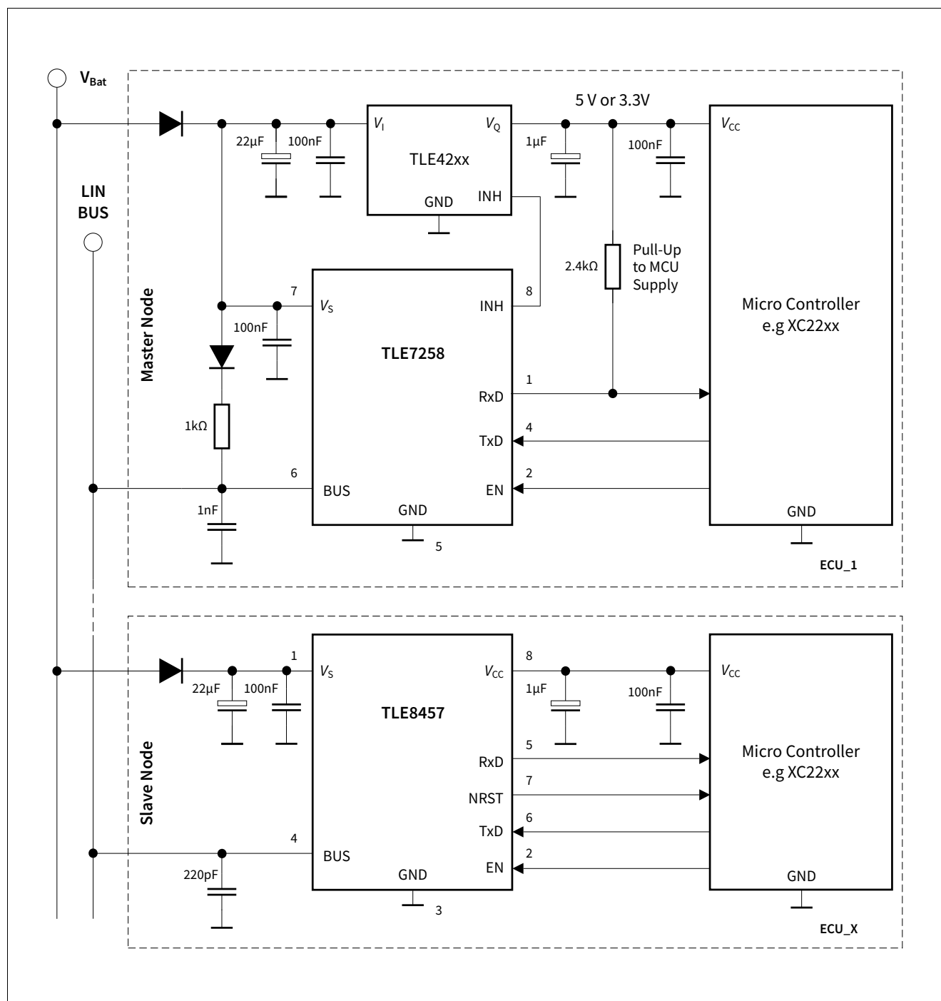
Figure 18 Simplified application circuit
