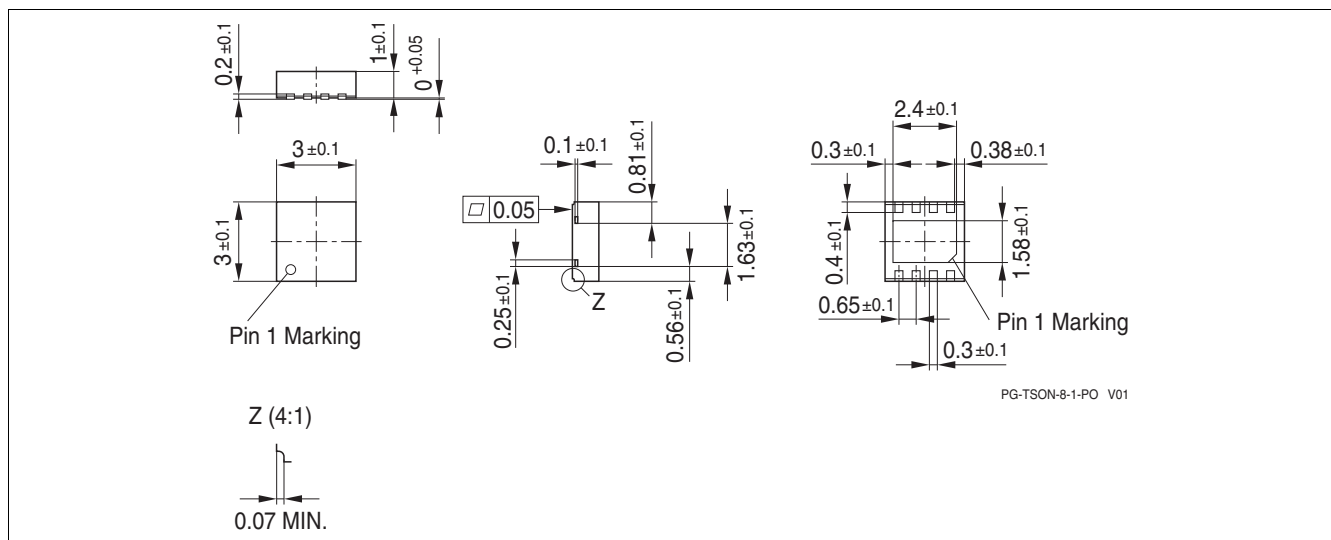
Figure 20 PG-TSON-8 (Plastic Thin Small Outline Nonlead PG-TSON-8)
