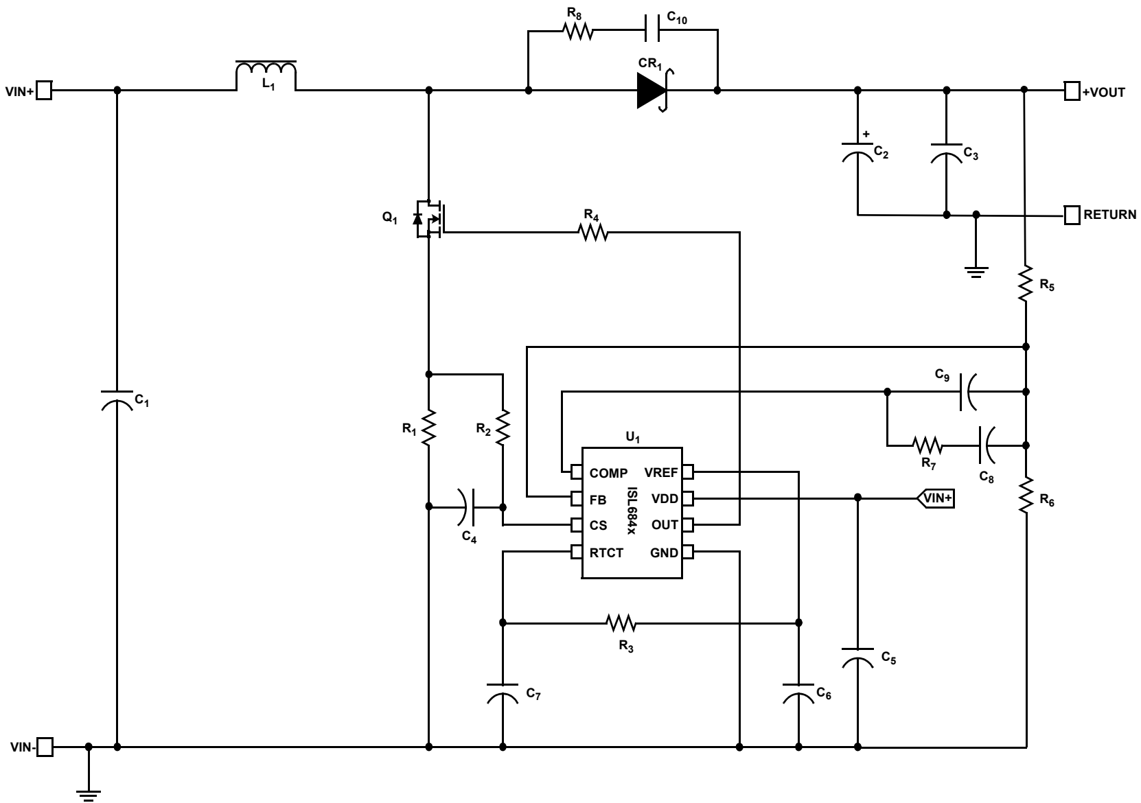
Figure 2. Boost Converter
