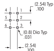
On-None-On Double Pole Models
