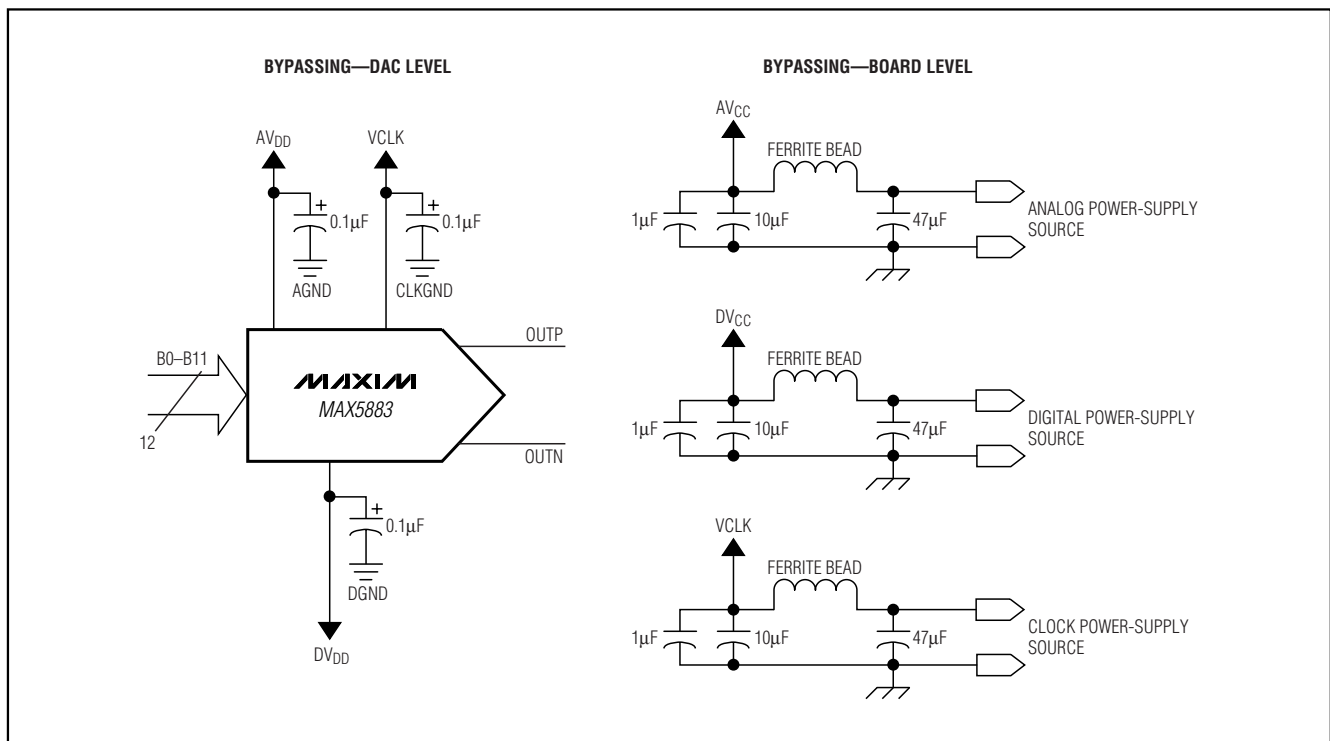
Figure 10. Recommended Power-Supply Decoupling and Bypassing Circuitry
