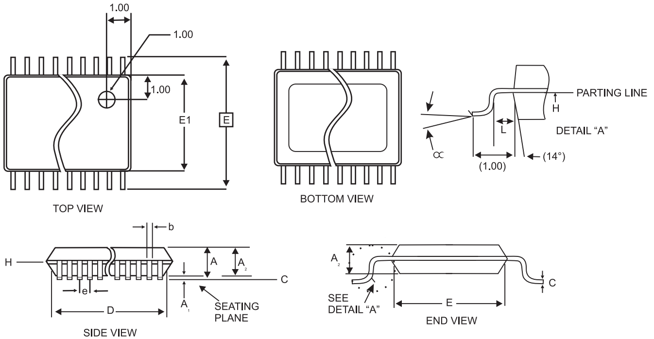
240 mil (6.10mm)TSSOP Package
