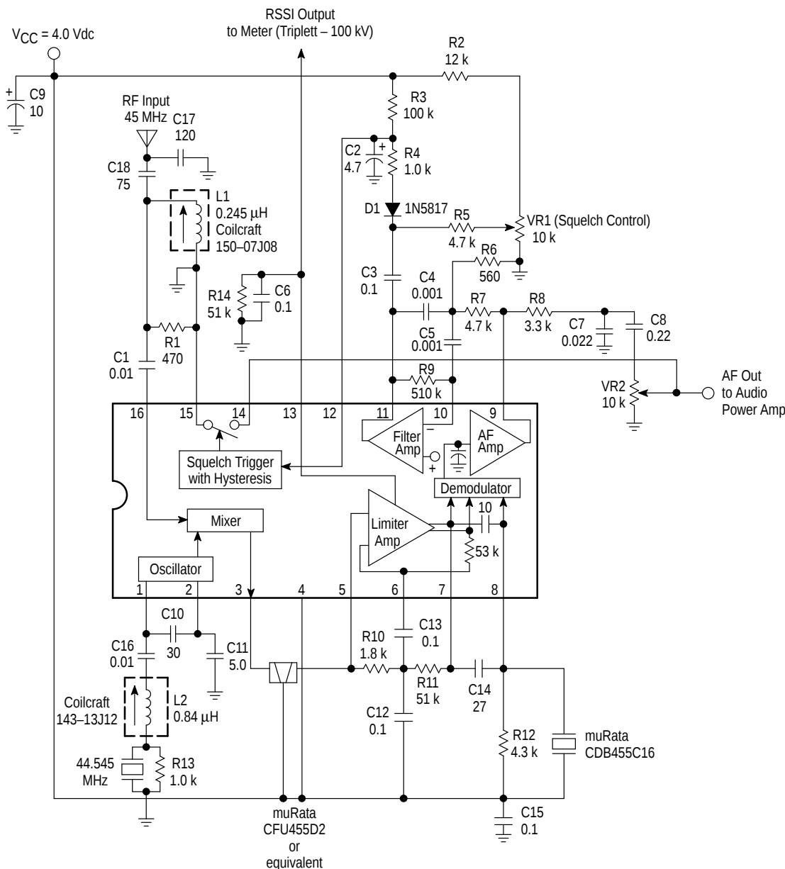
Figure 13. Typical Application for MC3372 at 45 MHz
