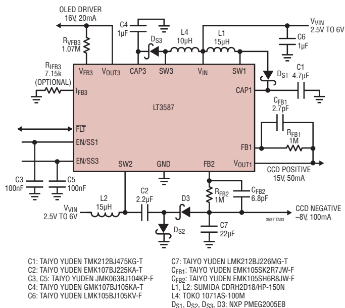
Driver For a CCD Imager and an OLED Display Panel with Soft-Start
