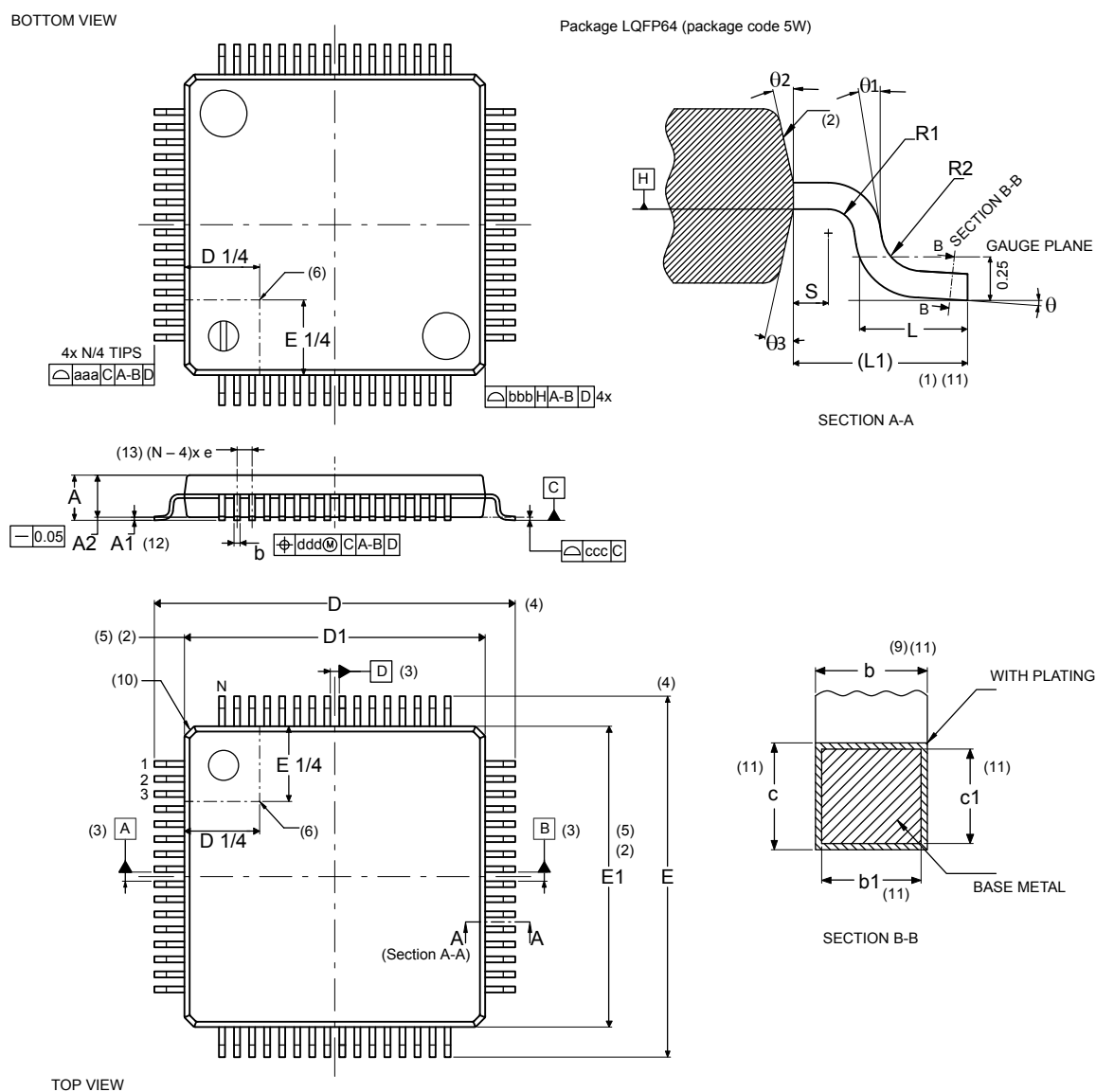
Figure 82. LQFP64 - Outline (15.)
