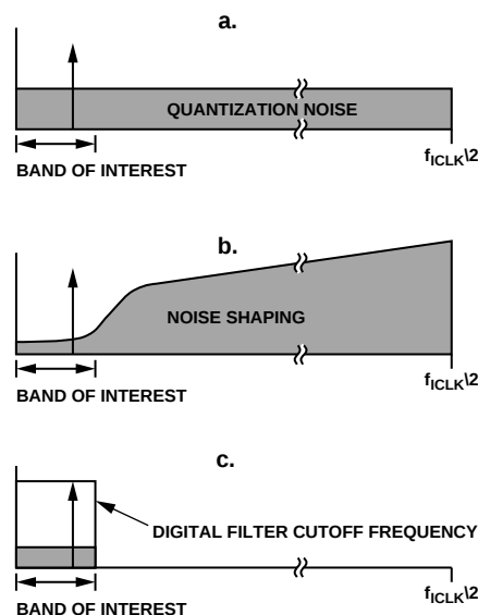
Figure 22. \Sigma - \Delta ADC
