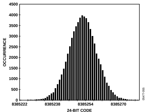
Figure 17. Normal Mode, 24-Bit Histogram, 256x Decimation
