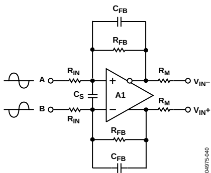
Figure 25. Differential Amplifier Configuration
