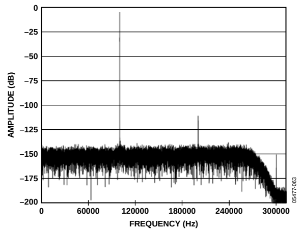
Figure 14. Low Power FFT, 100 kHz, -0.5 dB Input Tone, 32× Decimation
