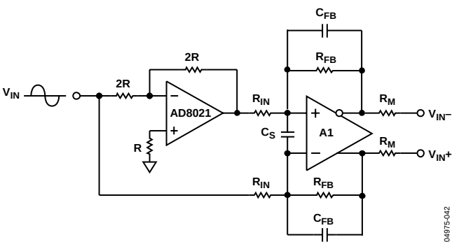
Figure 27. Single-Ended-to-Differential Conversion
