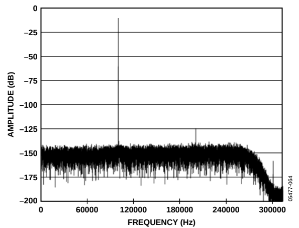
Figure 15. Low Power FFT, 100 kHz, -6 dB Input Tone, 32× Decimation
