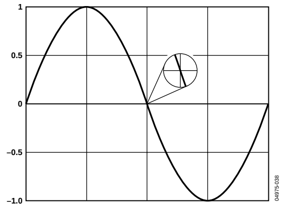
Figure 23. Maximum Slew Rate of Sine Wave with Amplitude of 2 V p-p
