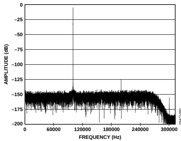
Figure 11. Normal Mode FFT, 100 kHz, -0.5 dB Input Tone, 32× Decimation
