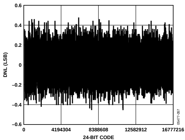
Figure 19. 24-Bit DNL
