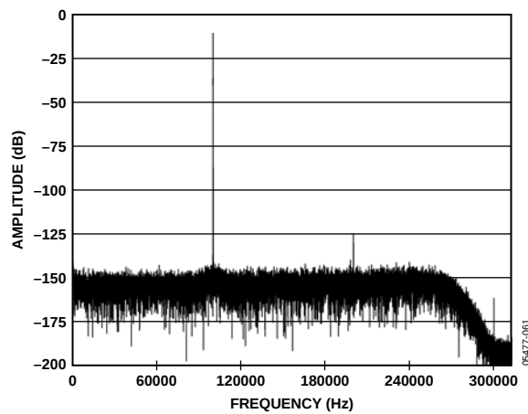
Figure 12. Normal Mode FFT, 100 kHz, -6 dB Input Tone, 32× Decimation
