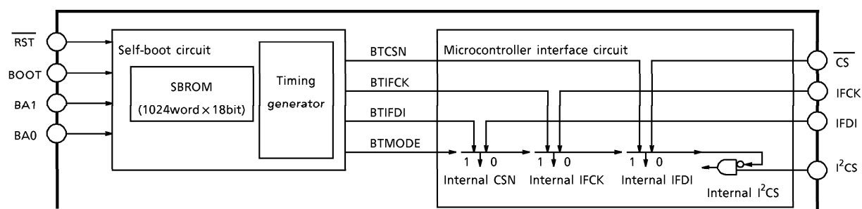
Fig.1 Self-Boot System
