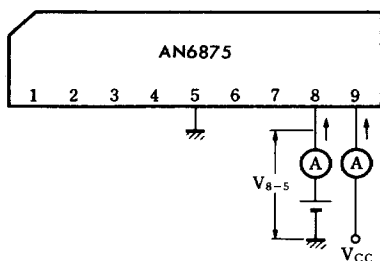
Test Circuit 1 ( I_{I1}, I_{I2}, I_{tot} )
