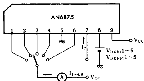
Test Circuit 2 ( V_{I(ON)1-5}, V_{I(OFF)1-5}, I_1 \sim I_4, I_6 )
