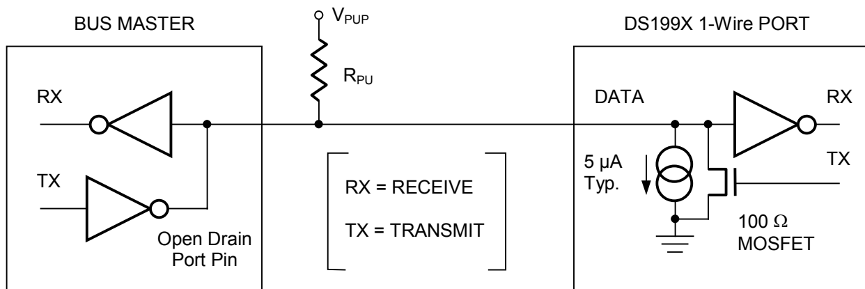
Figure 8. HARDWARE CONFIGURATION
