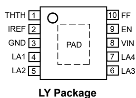
LY Package
