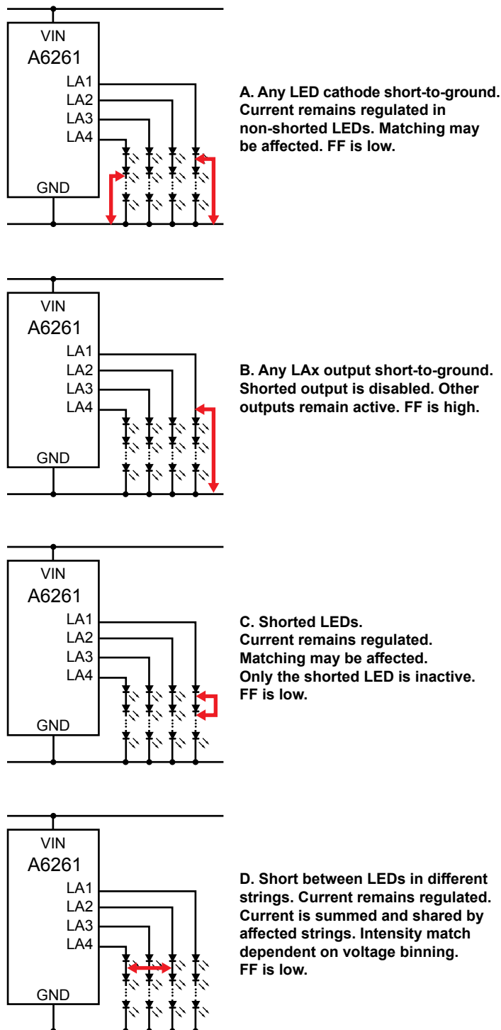
Figure 1: Short-Circuit Conditions
