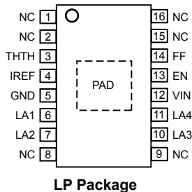
LP Package
