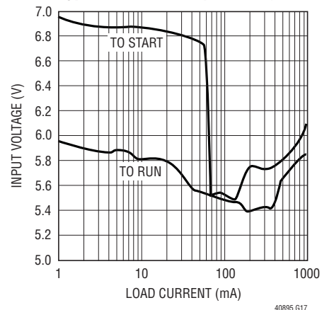
High Voltage Regulator Typical Minimum Input Voltage
