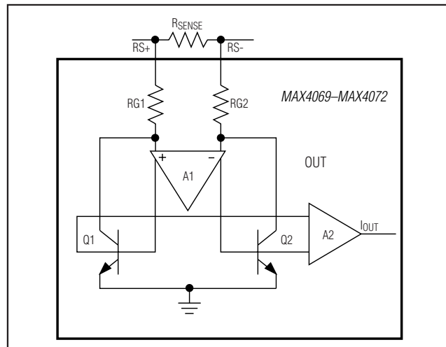
Figure 1. Detailed Input Stage
