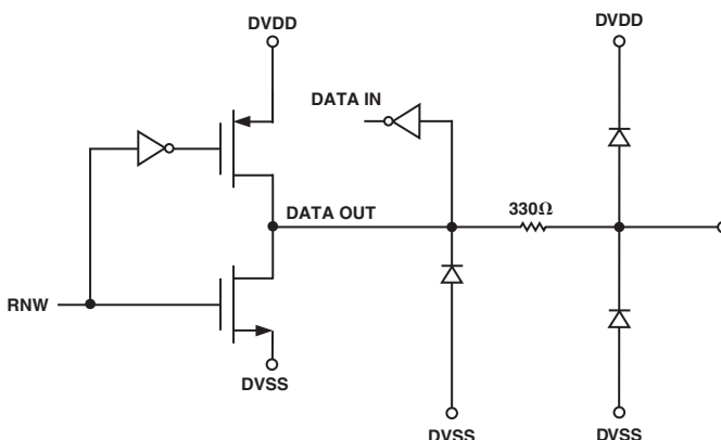
Figure 4. SDATA (Pin 47)
