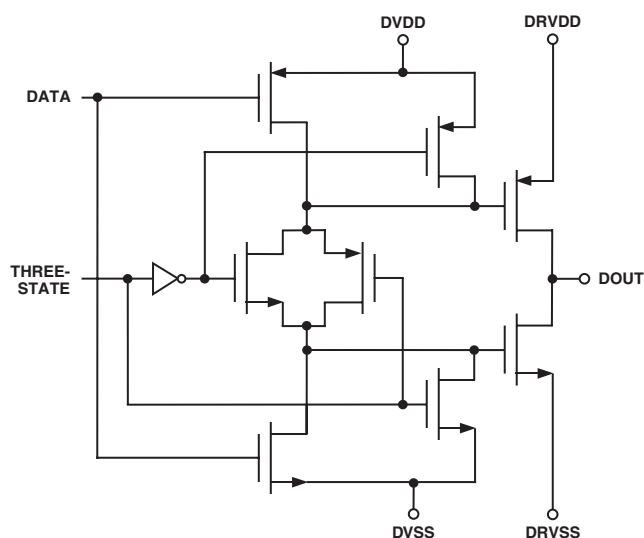
Figure 2. Data Outputs—D0–D11
