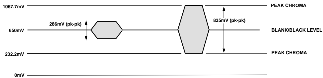
Figure 46. NTSC Chroma Video Levels
