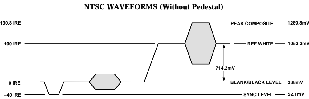
Figure 48. NTSC Composite Video Levels
