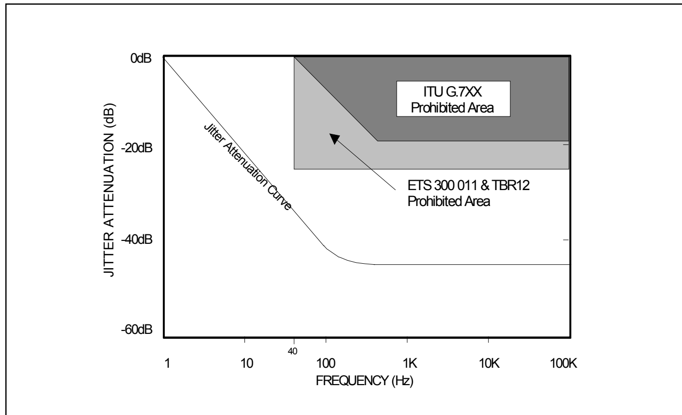
Figure 15-4. Jitter Attenuation
