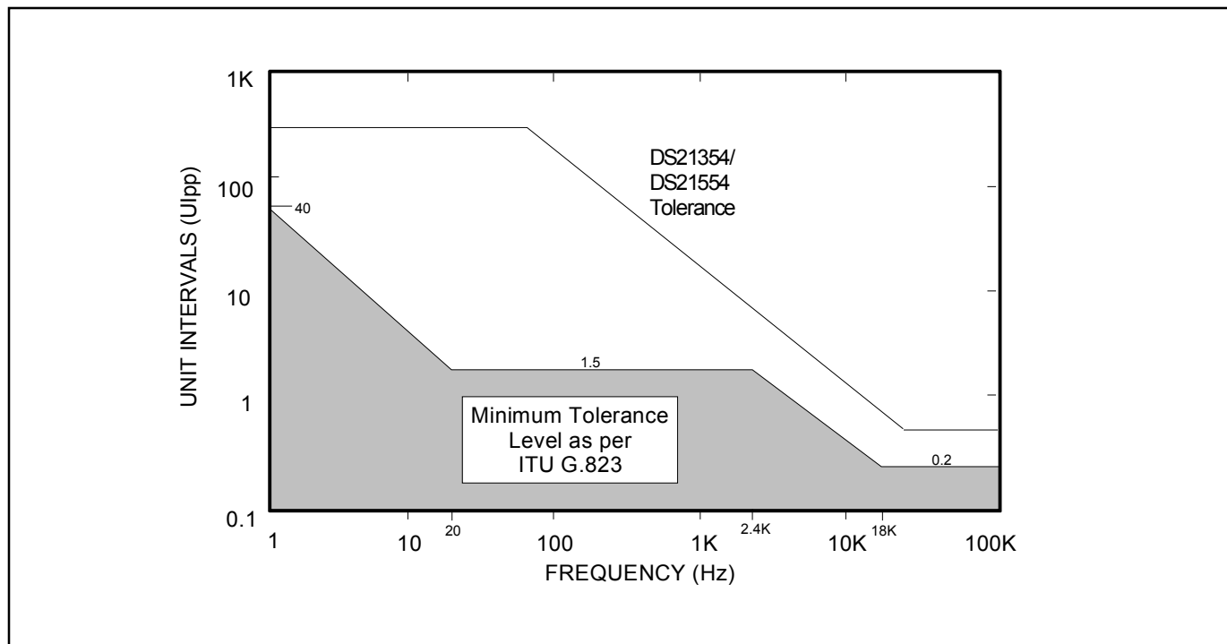
Figure 15-3. Jitter Tolerance
