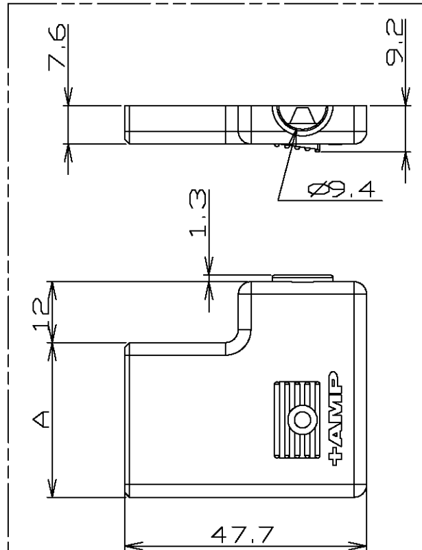
② COVER "B"
