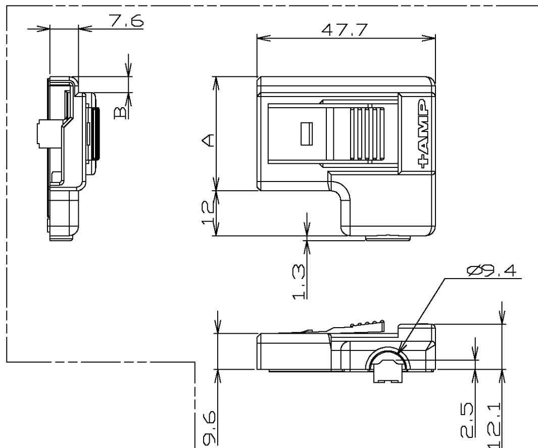
① COVER "A" (KEY "B")
