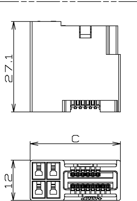
⑥ PLUG ASSEMBLY
