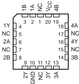
SN54HC7032 . . . FK PACKAGE (TOP VIEW)
