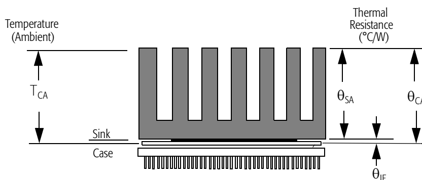
Figure 98. Thermal Model
